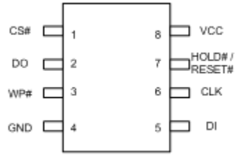
Figure 3.1 8-pin SOP 150/208mil (300mil)
