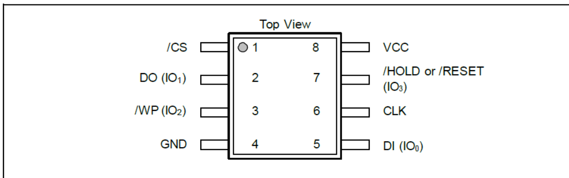
Figure 3.1 8-pin SOP (150/208mil) VSOP 208mil
