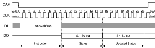
Figure 7.1a Read Status Register Instruction(SPI Mode)
