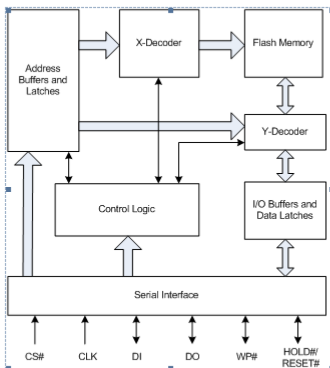
Figure 2.1 Block Diagram
