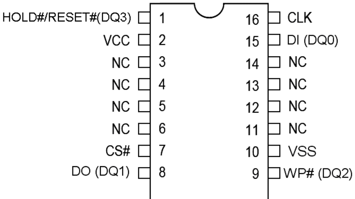
16 - LEAD SOP
