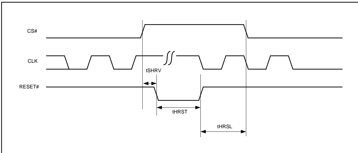
Figure 44. Reset Timing
