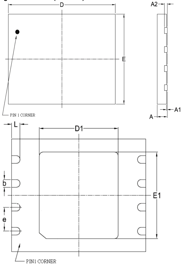
Figure 50. VDFN 8 ( 6x8 mm )
