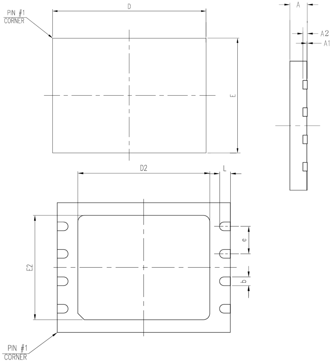
Figure 46. VDFN8 ( 5x6mm )
